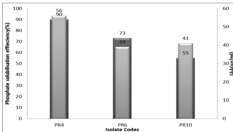
Fig 3: Graph of phosphate solubilization efficiency and Indole Acetic acid production by the heavy metal and salt tolerant isolate
