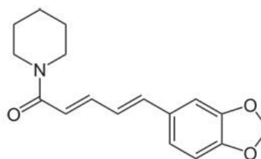
Fig 3: Structure of piperine
